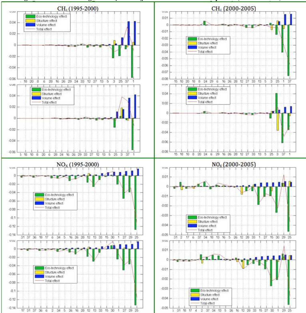
Figure D.2. SDA for changes in CH 4 and NO x emissions for the two sub-periods (PBA and CBA)
