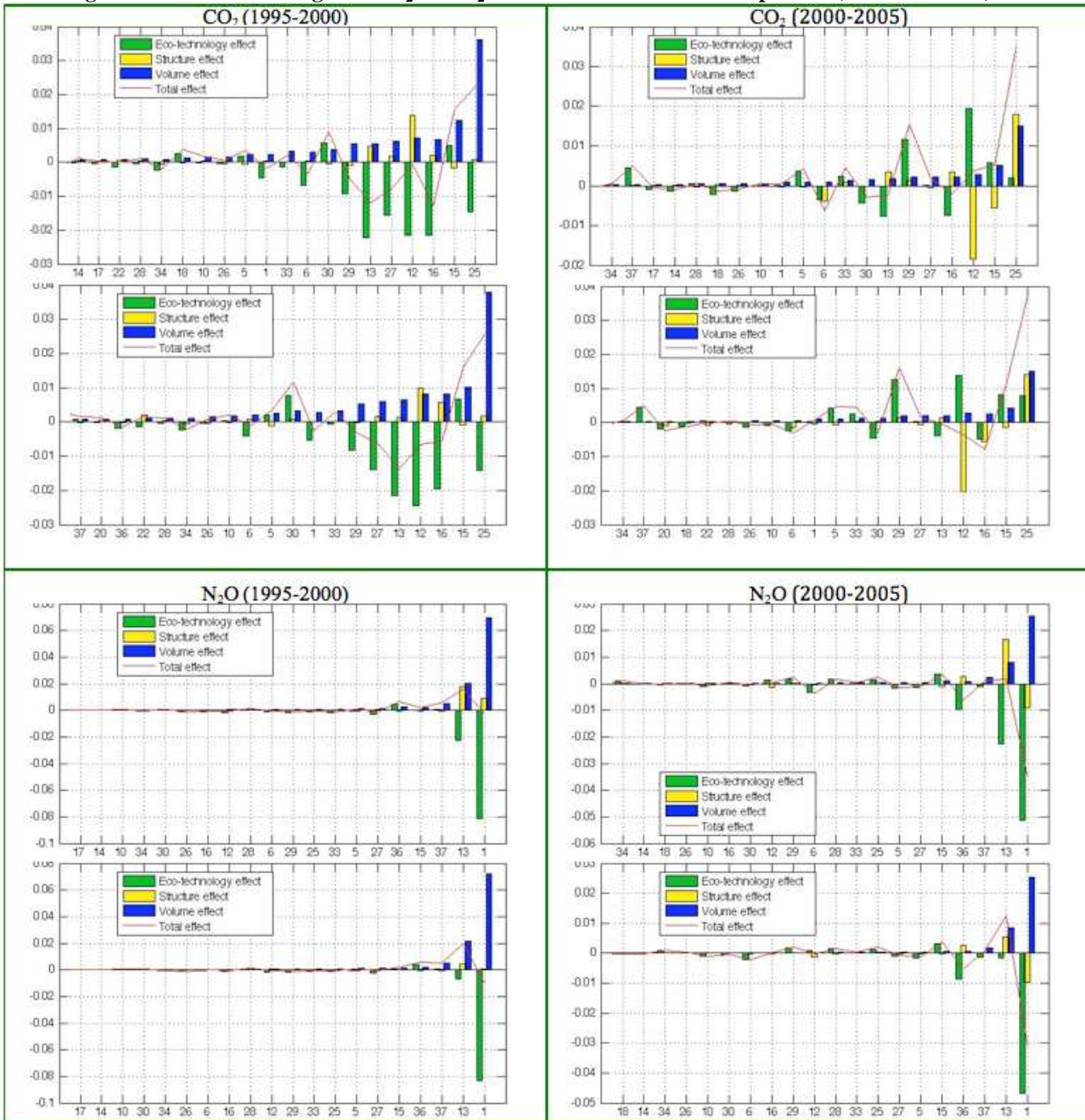
Figure D.1. SDA for changes in CO 2 and N 2 O emissions for the two sub-periods (PBA and CBA)
